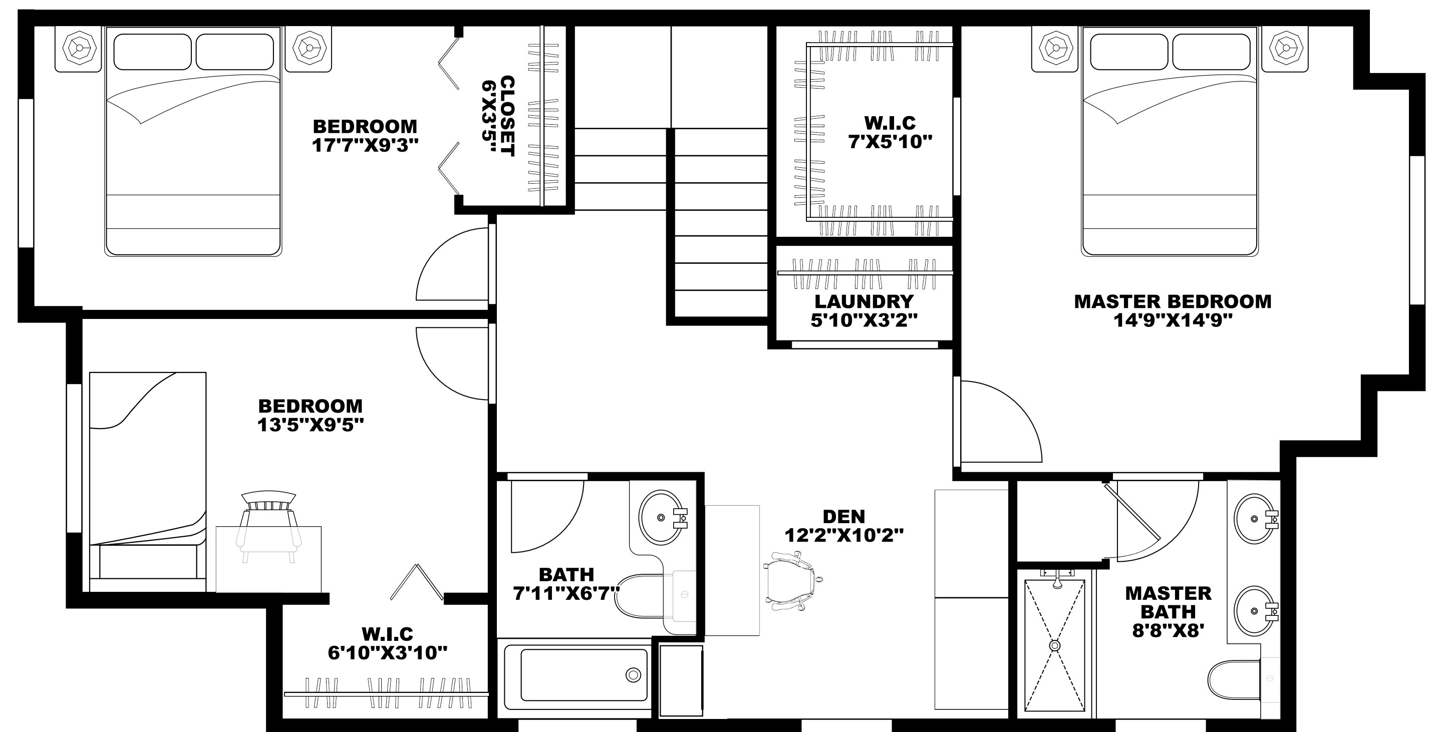
UPPER FLOOR
